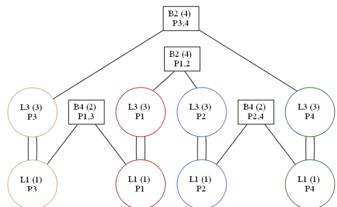
Fig. 2. Generated MLML. Numbers in braces identifies the corresponding LML zones. Each zone contains information about accessing them players.
